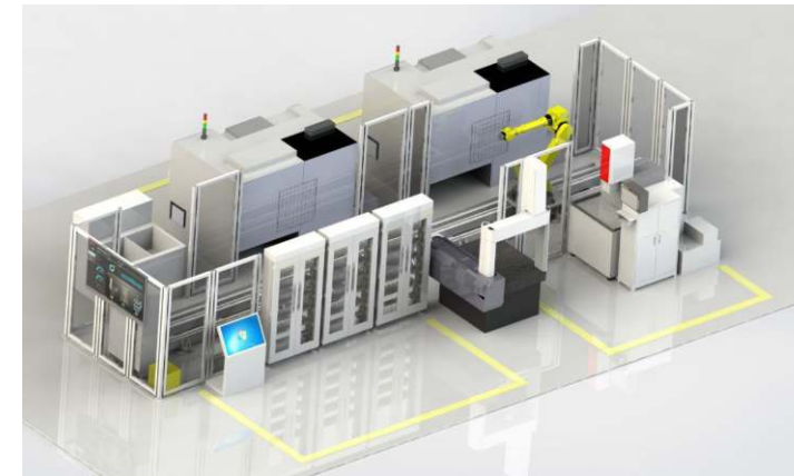
电极模具柔性制造自动化单元 Electrode die flexible manufacturing automation unit
