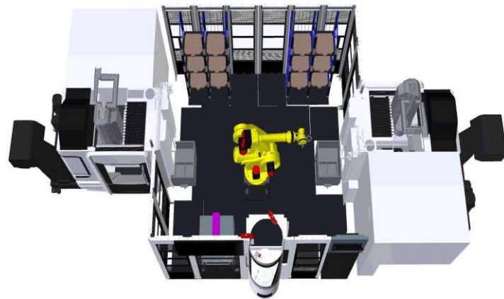
车铣组合自动化单元 Turn-milling combined automation unit
