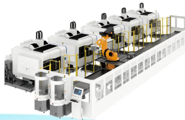
精密数控机床+自动化线+CAM软件+信息化系统 Precision CNC machine tool + automation line +CAM software+ Information system
